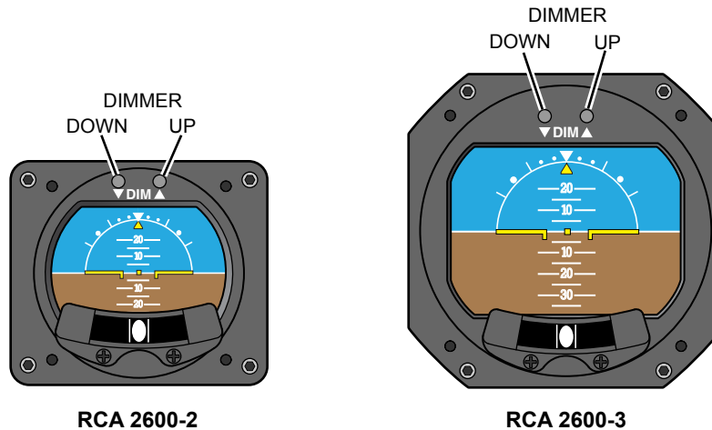
Figure 3.1, Dimming Controls
